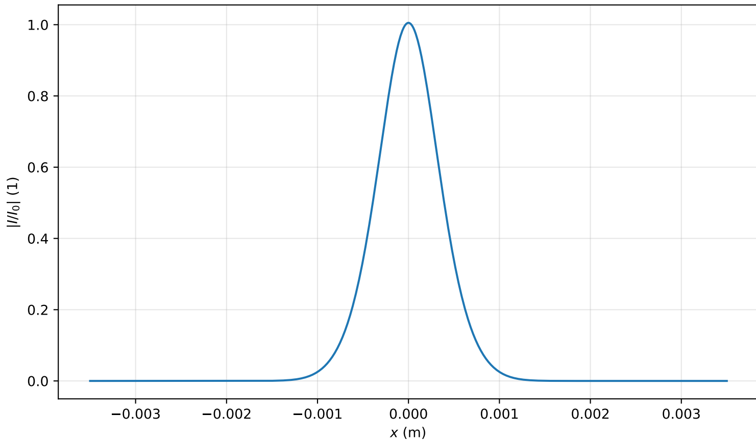
Intensity profile I(x, y = 0, z = 0.876m)/I_0 , P_{in}=0.4P_{cr} , artificial time
